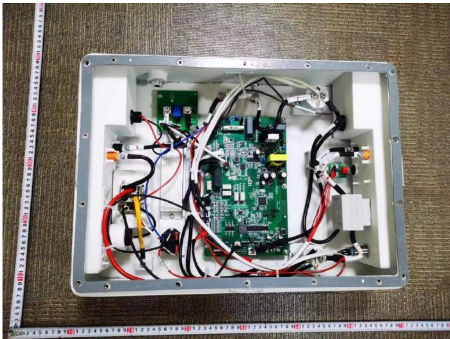
Inside of Main control unit, Model: TBMS-MCS0800
